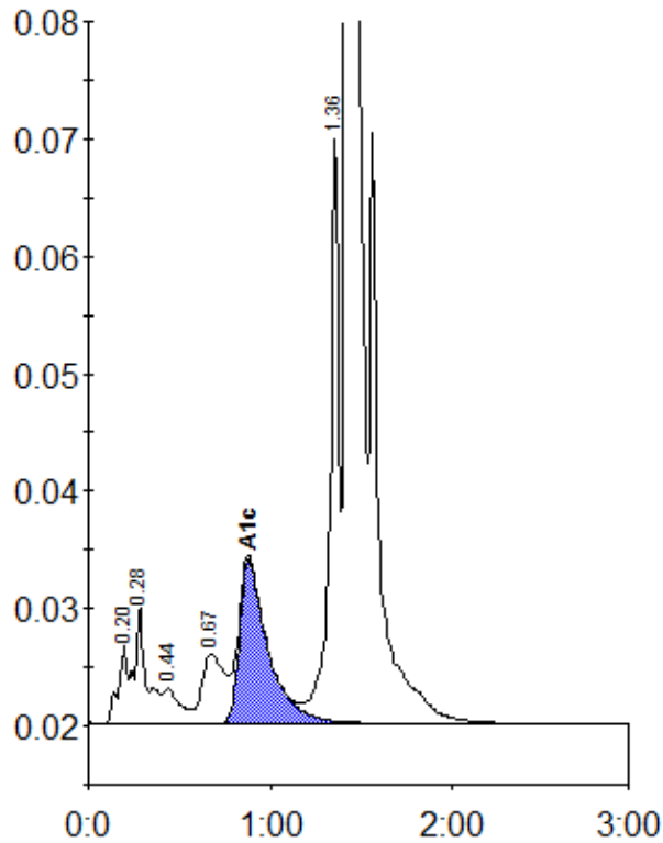
Peak table - ID: 10575327
